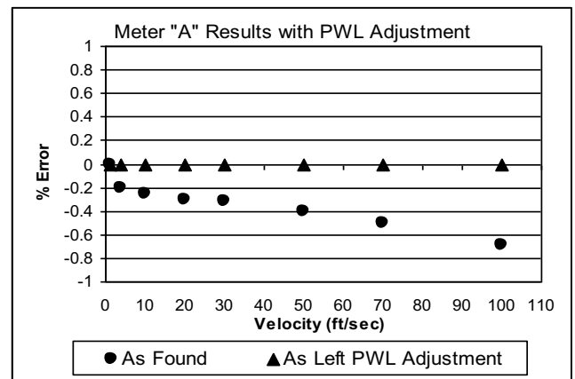
Figure 4. Meter “A” Results with Multi-Point Adjustment Applied.
