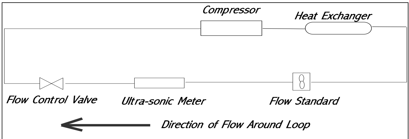
Drawing 2. Pressurized Loop Based Calibration Facility.
