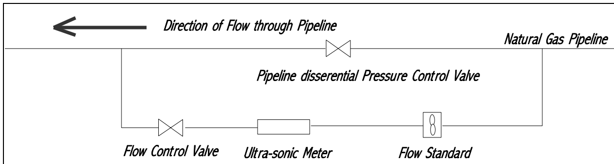
Drawing 1. Pipeline Based Calibration Facility.
