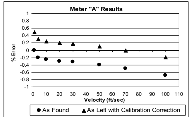
Figure 1. Meter "A" Results with Correction Applied.
