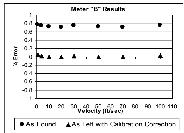
Figure 2. Meter "B" Results with Correction Applied.
