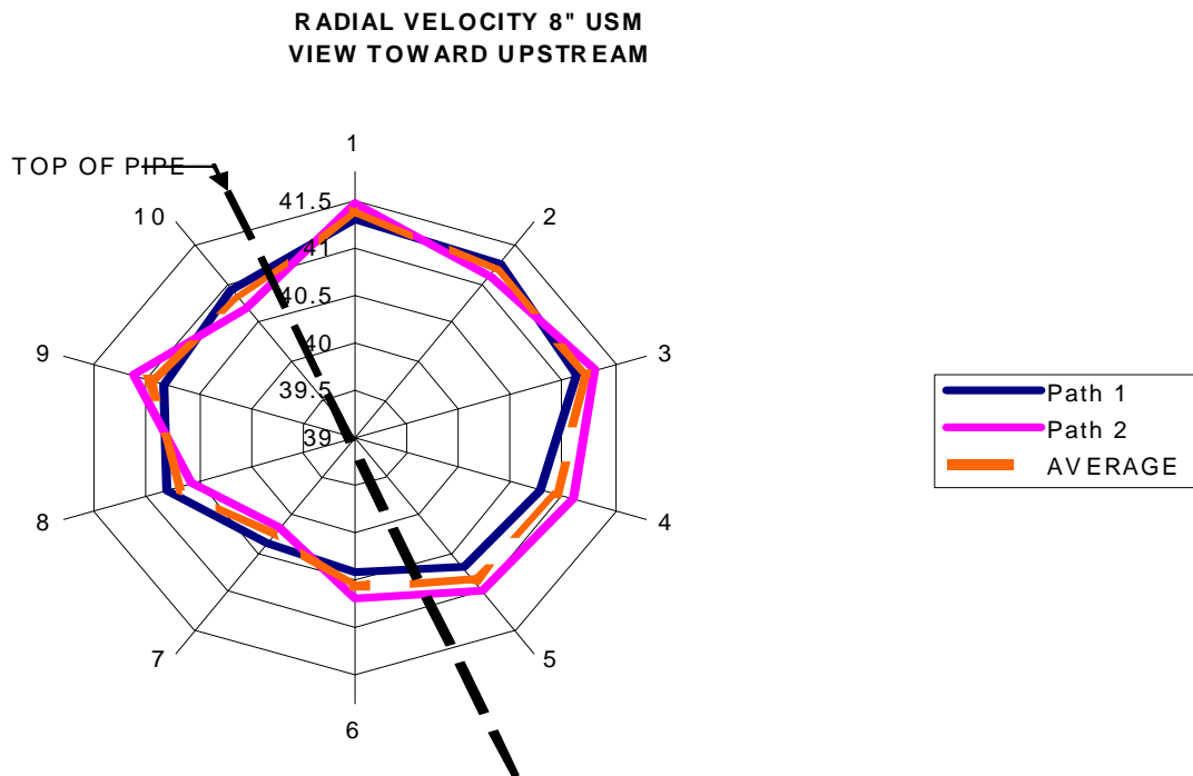
Figure V. Polar Plot of Profile Distortion Segmentation Check Meter
