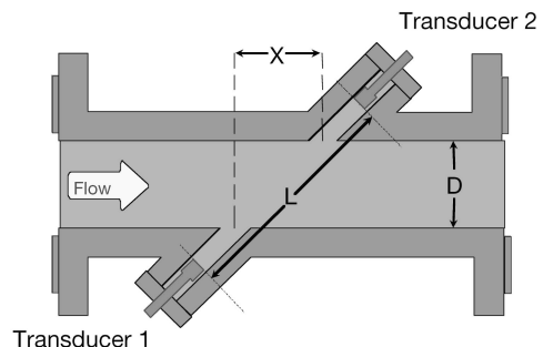
FIGURE 1. Ultrasonic Flow Meter
