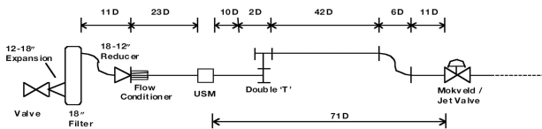
FIGURE 5 – Better USM Piping Diagram
