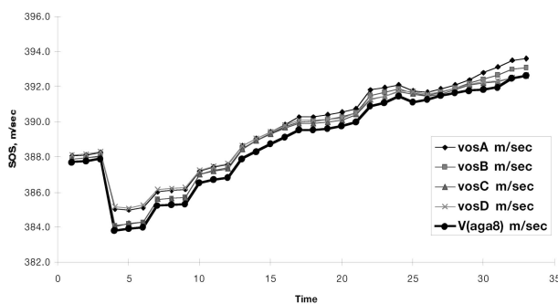
FIGURE 3. 10-inch Meter SOS with 4 Chords
