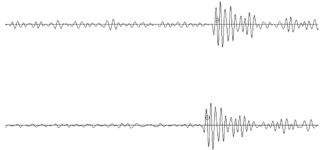
GRAPH NO. 1 – Typical USM Waveform
