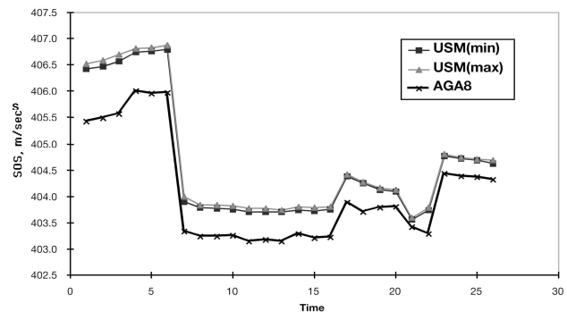
FIGURE 2. 8-INCH METER MEASURED VS. CALCULATED SOS
