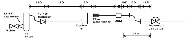
FIGURE 4. Poor USM Piping Diagram
